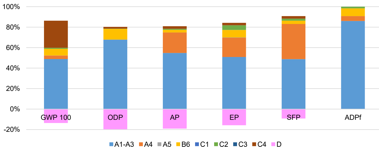
Figure 3: Contributions to the environmental impact categories for copper patch cord Cat 6/6A
