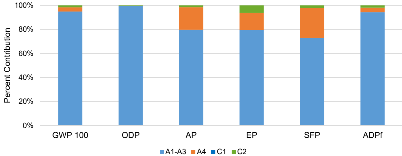
Figure 5: Contributions to the environmental impact categories for Cat 6A field termination plug
