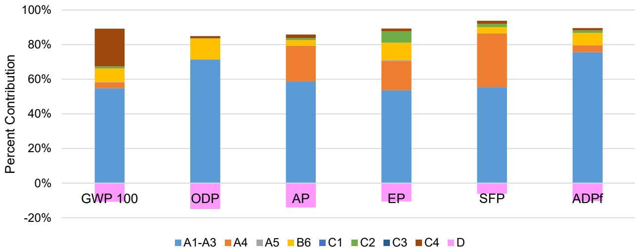
Figure 2: Contributions to the environmental impact categories for copper small diameter high flex patch cord Cat 6/6A
