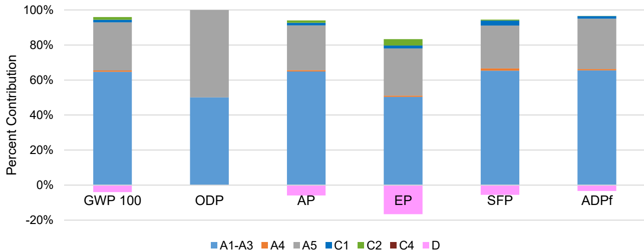
Figure 4: Contributions to the environmental impact categories for Cat 6/6A patch cord plug
